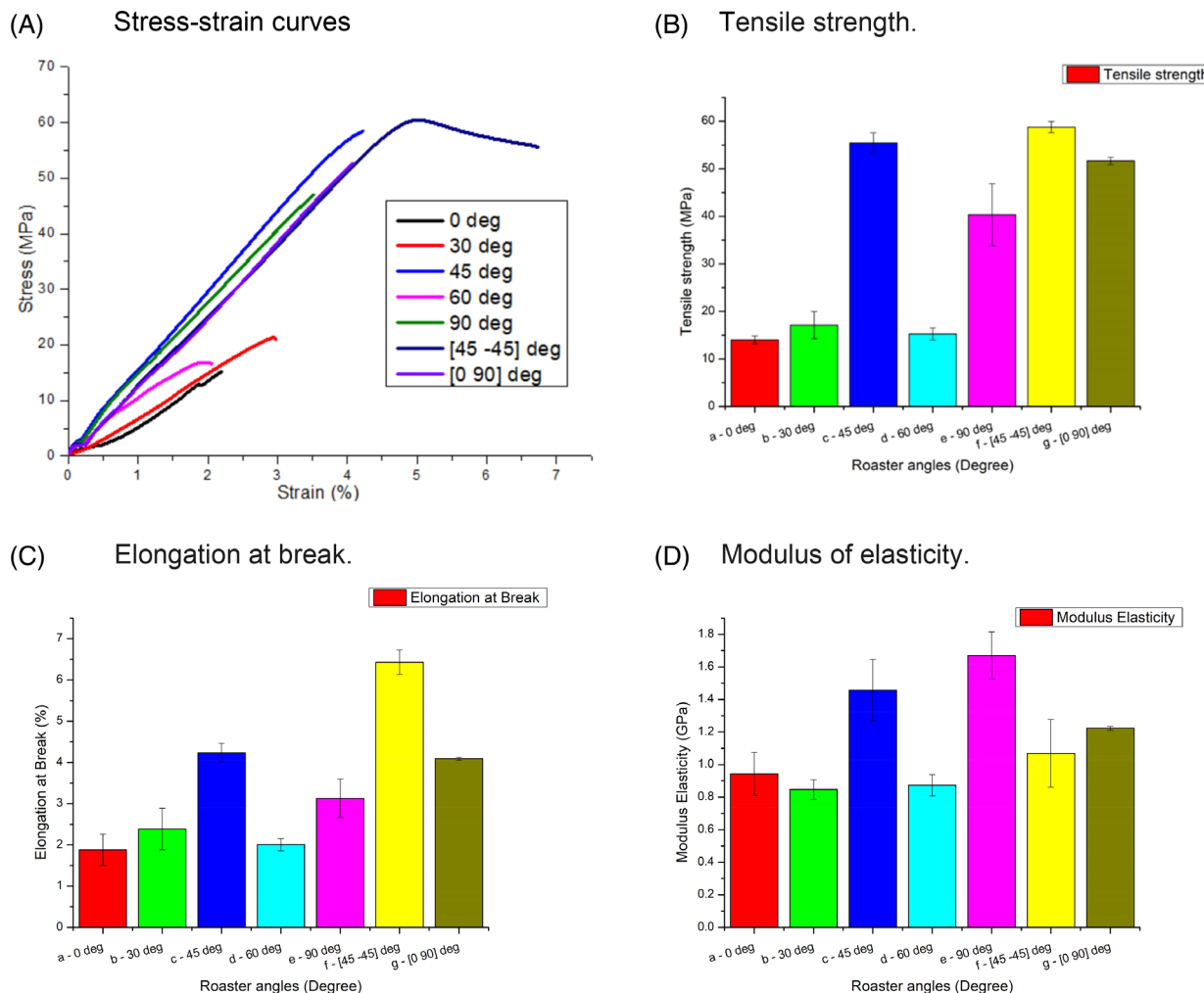
FIGURE 1 Material properties of 3D printed samples with seven different raster orientations in Experiment 1. (A) Stress–strain curves (B) Tensile strength. (C) Elongation at break. (D) Modulus of elasticity.
