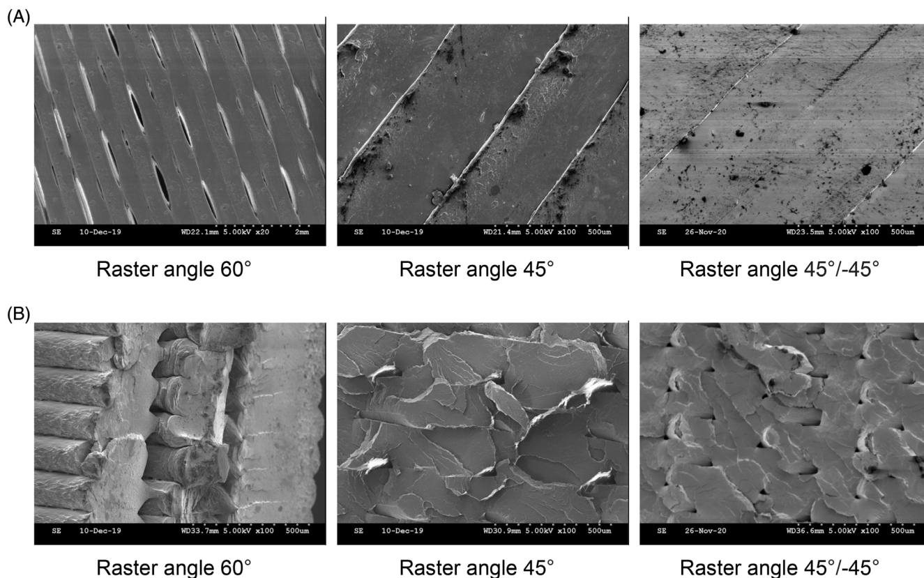
FIGURE 2 SEM images (A) outer surfaces and (B) fractured surfaces.
