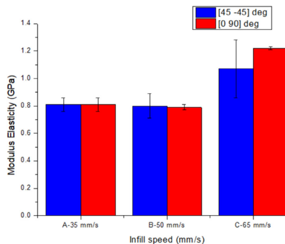
FIGURE 7 Modulus of elasticity.
