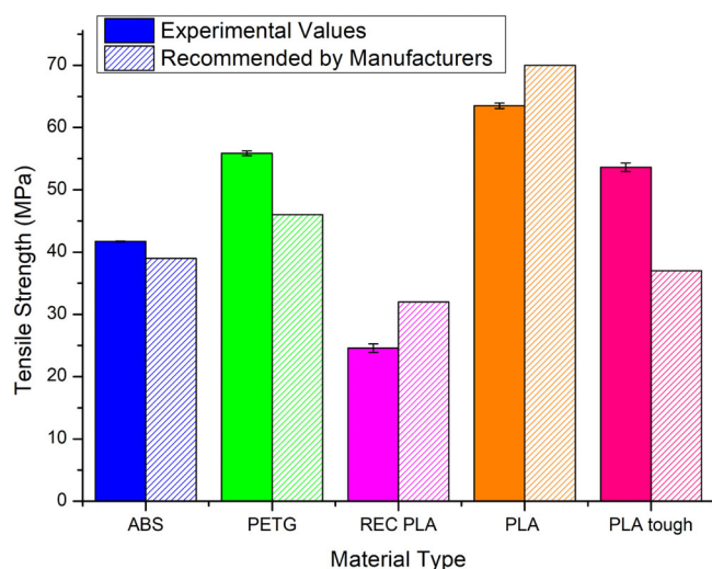
FIGURE 12 A comparison of tested tensile strength values against manufacturer-recommended values for the various materials.
