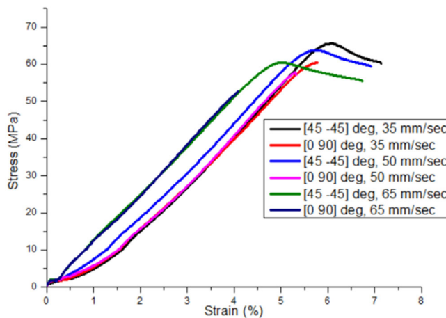
FIGURE 4 Stress-strain curves for all the samples.
