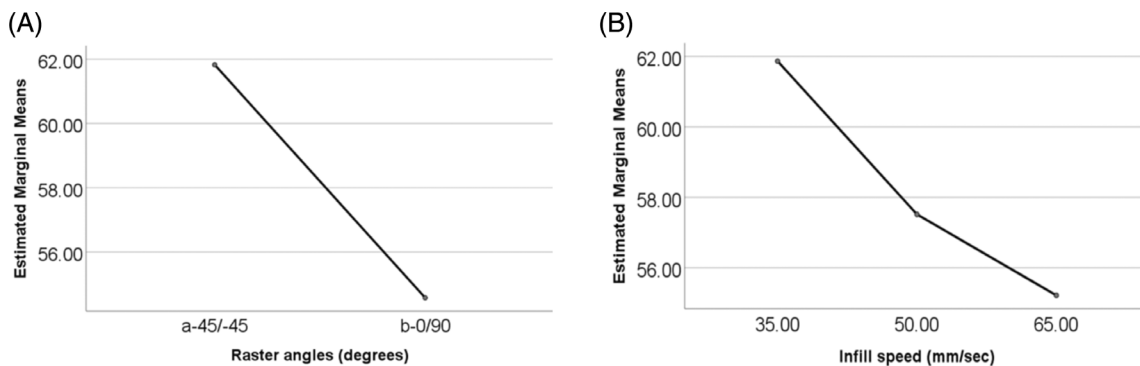
FIGURE 9 Main effect of 3D printing process parameters on tensile strength (A) Raster orientation (B) Infill speed.
