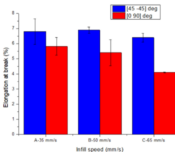
FIGURE 6 Value of elongation at break.
