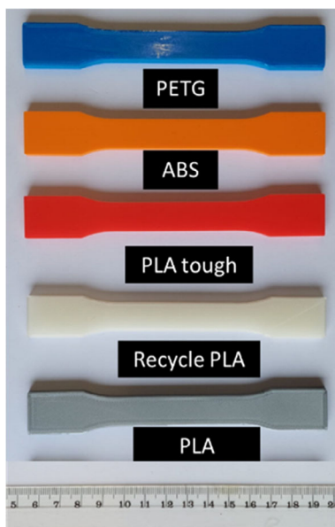
FIGURE 11 Tensile test samples for five different materials.
