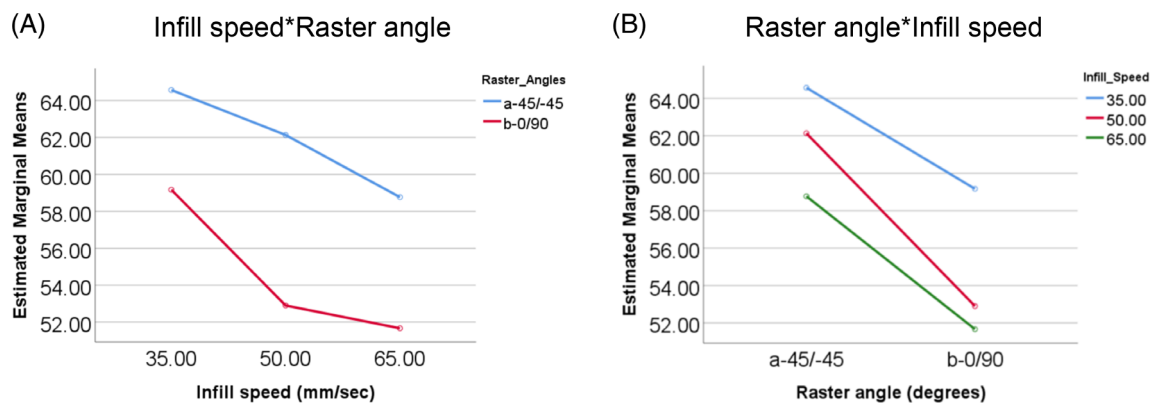
FIGURE 10 Interaction effort of process parameters on tensile strength. (A) Infill speed*Raster angle (B) Raster angle*Infill speed.
