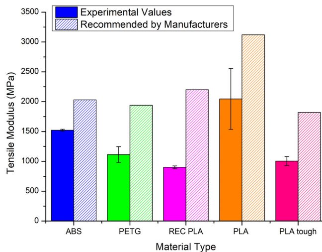
FIGURE 13 A comparison of tested Modulus of elasticity values against manufacturer-recommended values for the various materials.
