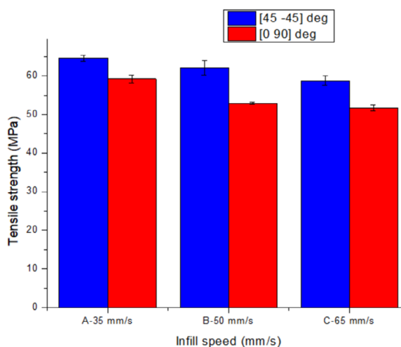
FIGURE 5 Tensile strength.
